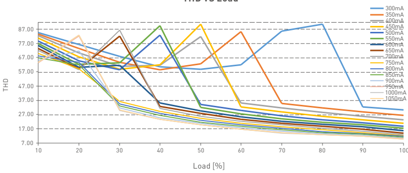
THD VS Load
