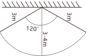
Ceilling mounting pattern(
