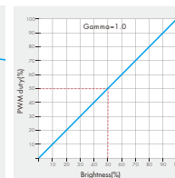
Dimming curve for CCT
