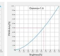
Dimming curve for RGB/DIM
